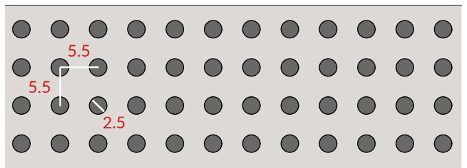
Perforated surface
